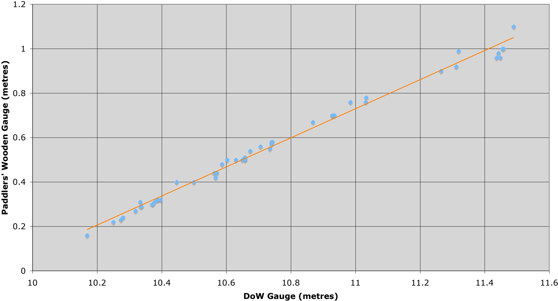
Comparison DoW and Wooden Gauges, Walyunga, 31st July, 2007
